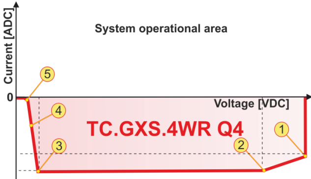
Q4 range of device TC.GXS.20.65.4WR.S.
