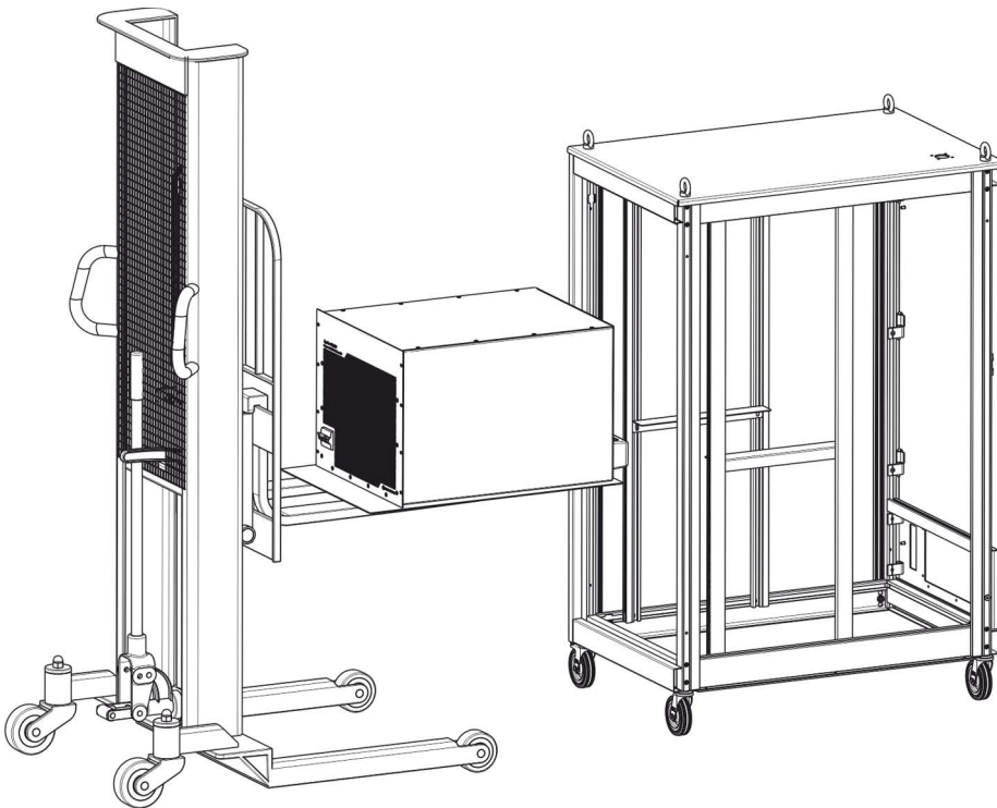
Fig. 11: Case installation with the help of a trolley
