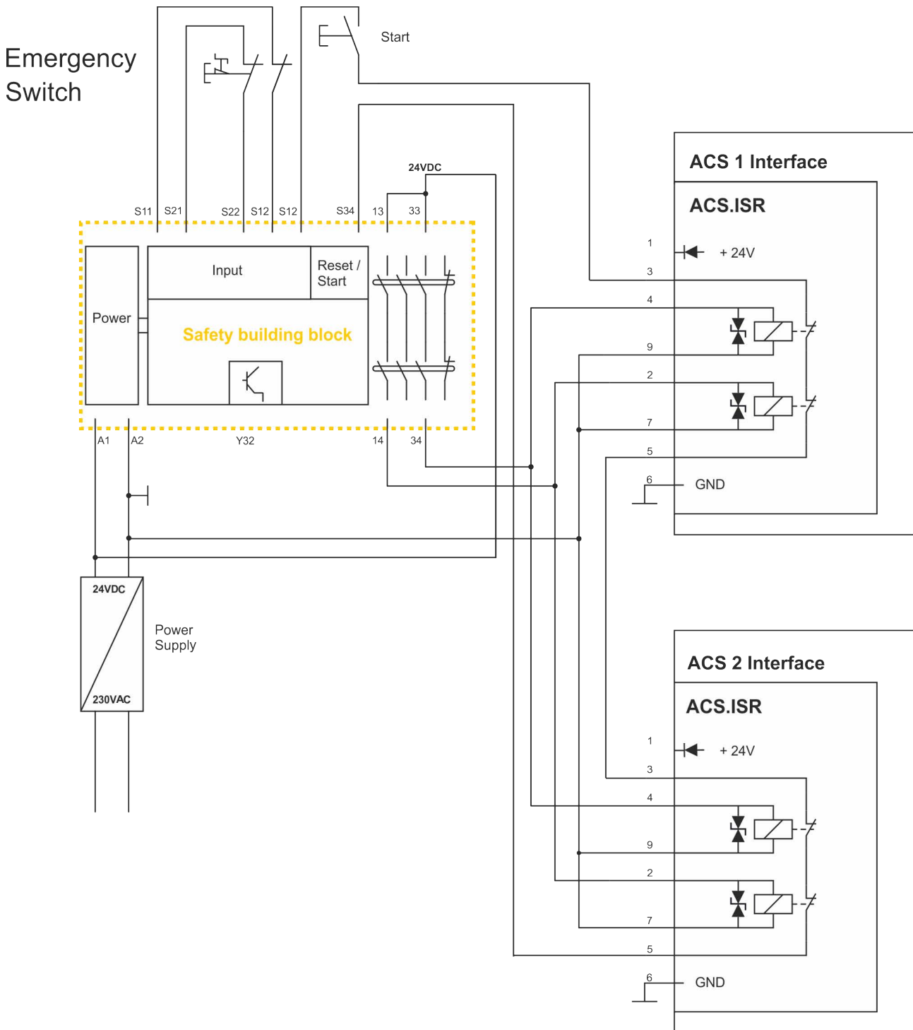
Fig. 10: Wiring diagram using an external safety module, two-channel safety loop
