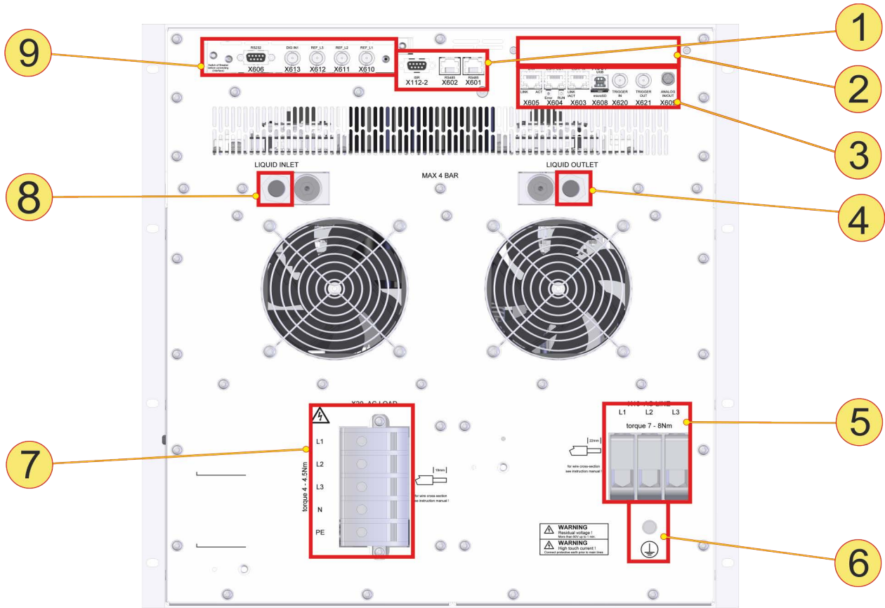
Fig. 6: Interfaces on the rear side
