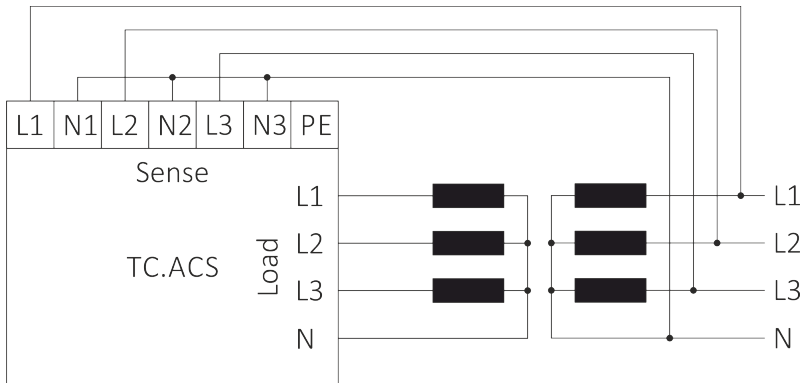
Fig. 16: Sense wiring for phase connection
