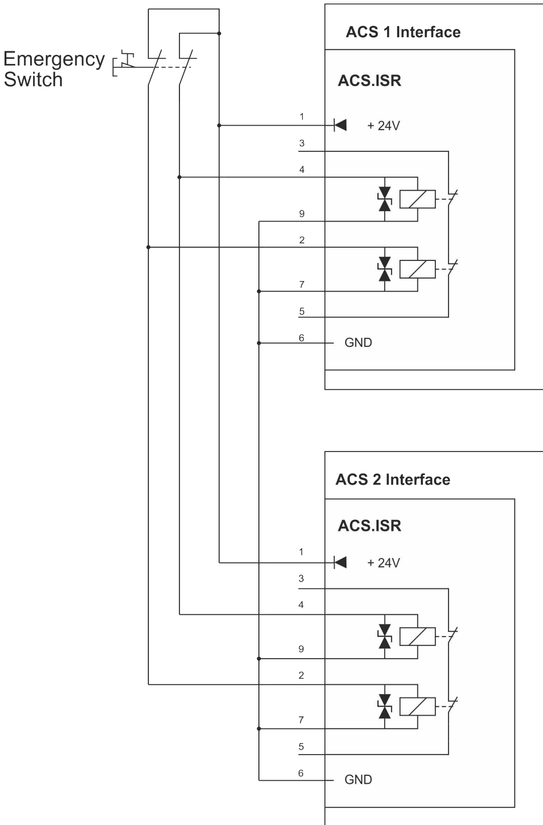
Fig. 9: Wiring diagram using a two-channel external safety loop
