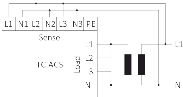
Fig. 17: Sense wiring for phase connection 1L (double current)
