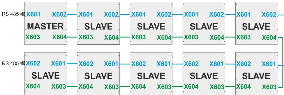
Fig. 13: Multi-device communication bus (green) and RS-485 bus (blue) connections in a TC.ACS multi-device system of 10 devices
