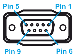
Fig. 7: Type of connection of interface X112-2: D-Sub, 9-pin, socket
