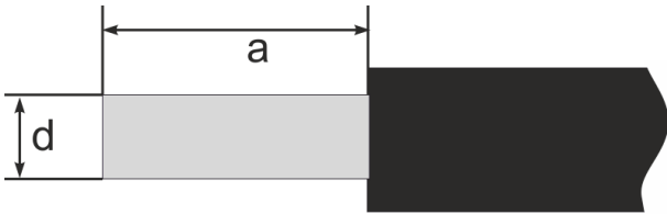
Fig. 12: Conductor end with diameter d and stripping length a
