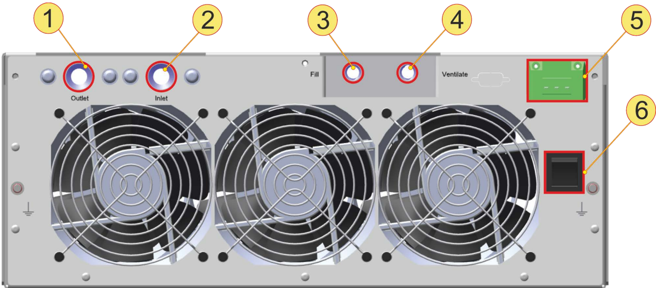
Fig. 23: Interfaces, controls and displays (rear side)
