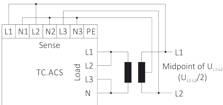
Fig. 18: Sense wiring for phase connection 2L (double voltage/double current)
