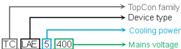
Fig. 21: Model identifier (example)
