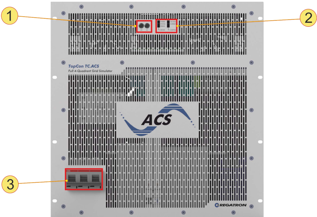
Fig. 5: Interfaces, displays and controls on the front side
