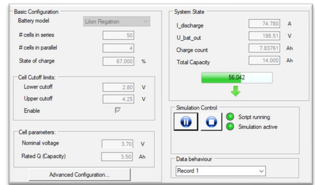
Figure 2: BATSIM configuration – a few clicks away from the required battery simulation.
