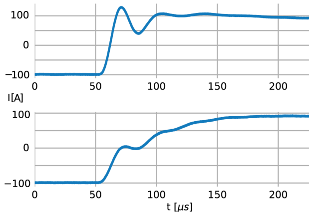
Figure 5: Parameterization example: of a 36 kW, 1000 V, 108 A device: Set-value step current -97...97 A@333VDC in <50 \mu s with overshoot (top), in <200 \mu s w/o overshoot (bottom). This dynamic behavior is characteristic for all G5 devices.
