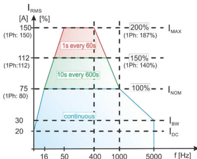
Figure 3: Overloadability vs. frequency (Phase Connection '3L (AC/DC)')
