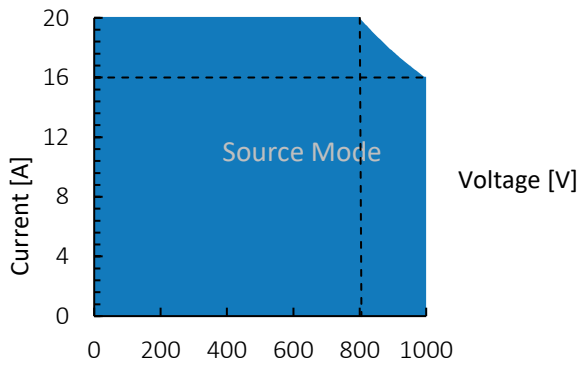
Figure 1: TC.P.16.1000.400.S, voltage / current operating area.
