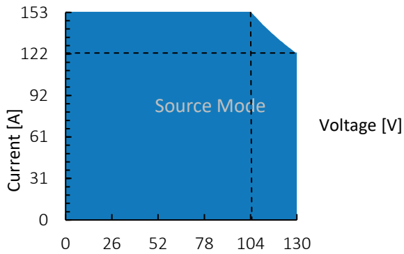
Figure 1: TC.P.16.130.400.S, voltage / current operating area.
