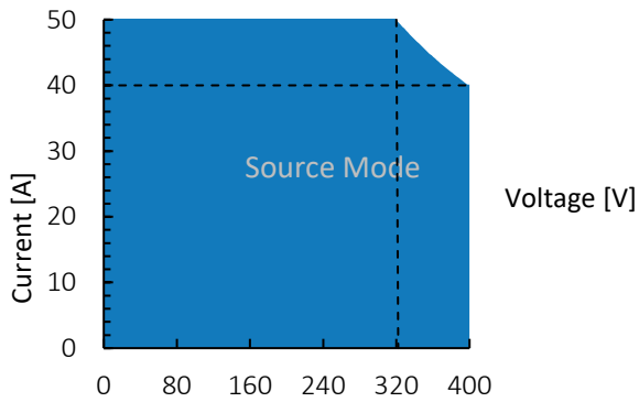
Figure 1: TC.P.16.400.400.S, voltage / current operating area.
