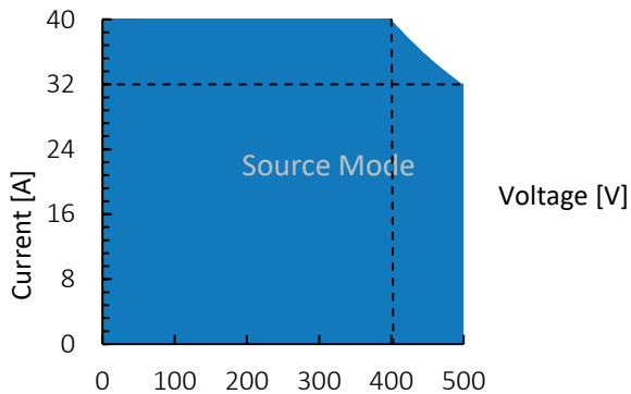
Figure 1: TC.P.16.500.400.S, voltage / current operating area.
