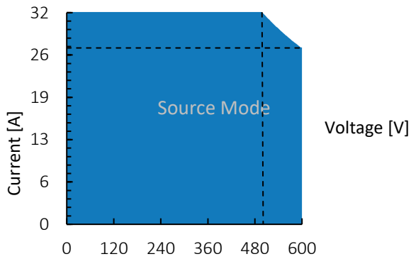
Figure 1: TC.P.16.600.400.S, voltage / current operating area.
