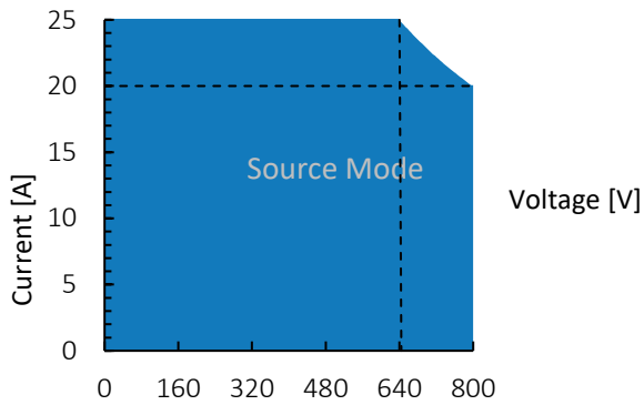
Figure 1: TC.P.16.800.400.S, voltage / current operating area.
