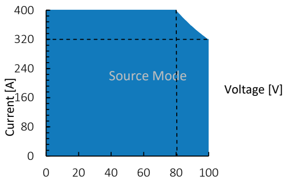
Figure 1: TC.P.32.100.400.S, voltage / current operating area.
