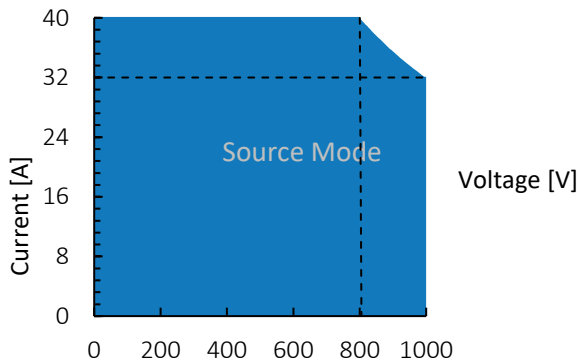
Figure 1: TC.P.32.1000.400.S, voltage / current operating area.
