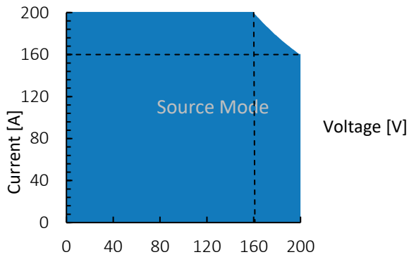
Figure 1: TC.P.32.200.400.S, voltage / current operating area.
