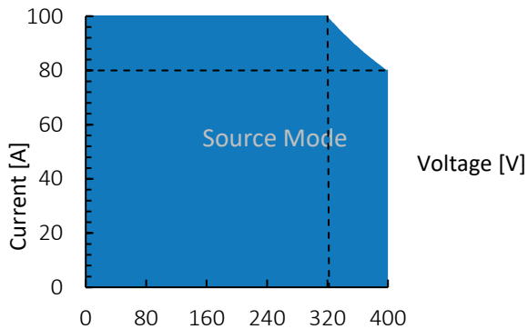
Figure 1: TC.P.32.400.400.S, voltage / current operating area.
