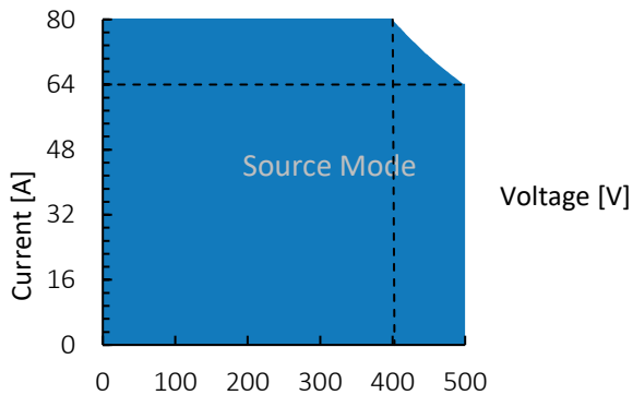
Figure 1: TC.P.32.500.400.S, voltage / current operating area.
