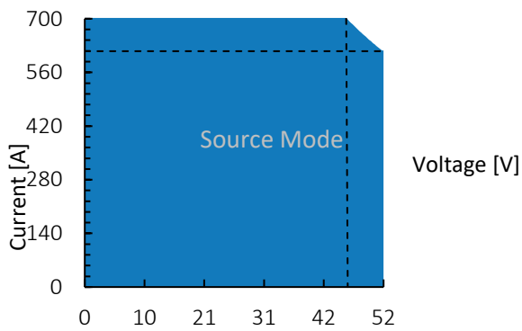
Figure 1: TC.P.32.52.400.S, voltage / current operating area.
