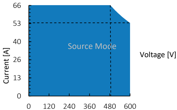
Figure 1: TC.P.32.600.400.S, voltage / current operating area.
