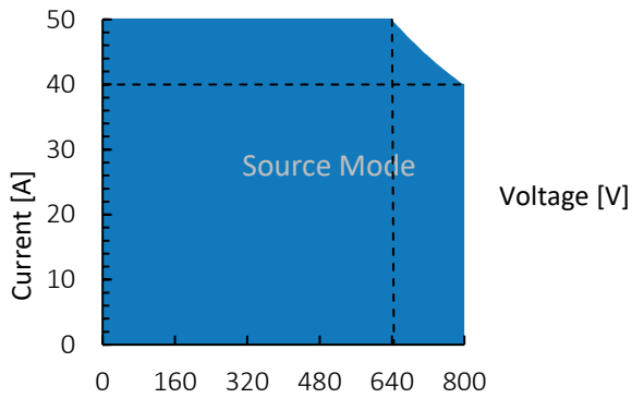
Figure 1: TC.P.32.800.400.S, voltage / current operating area.
