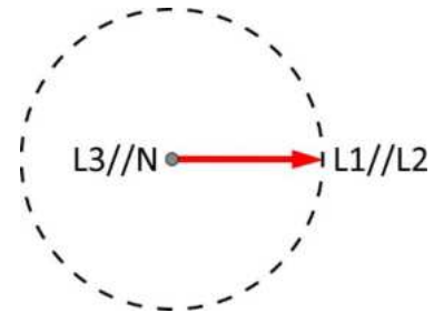
Figure 10: Phase Connection '1L (AC/DC double current)'
